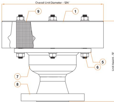
Corta-Chamas EVB: DN 15-40mm (1/2"-1.1/2")
