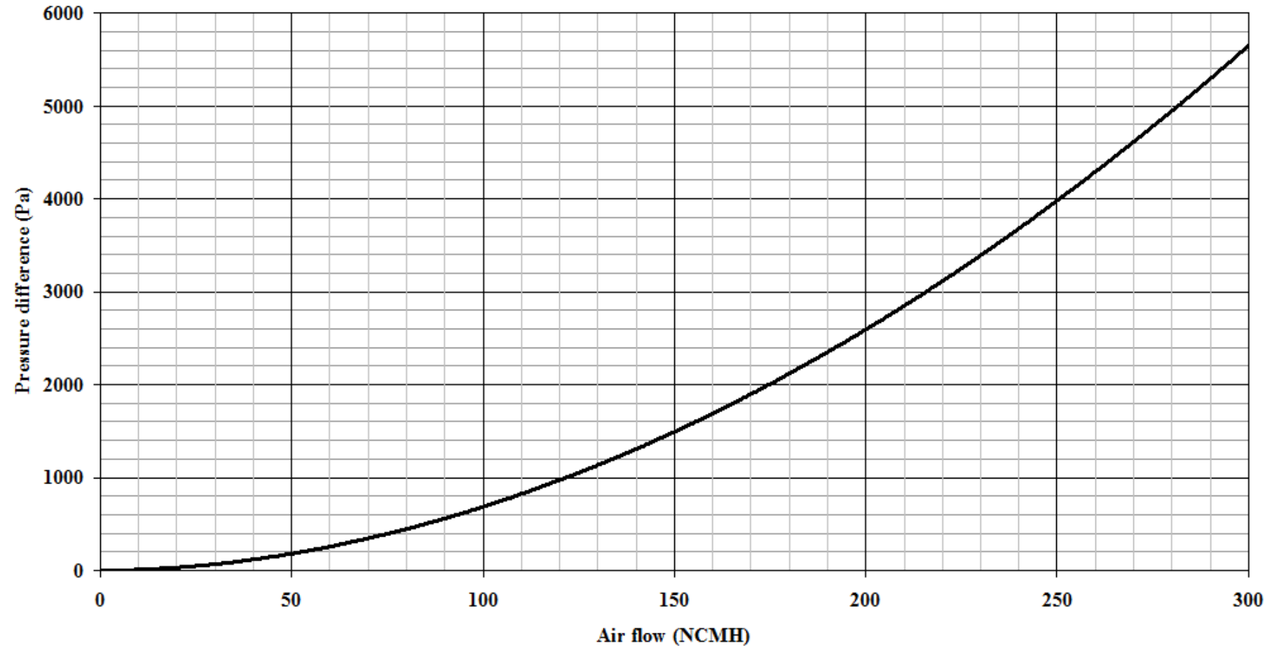
FE-IB-040 - Flow capacity of IIB3 deflagration flame arrestor
